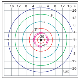
Isolux curve
