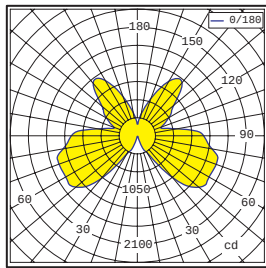
Photometric curve
