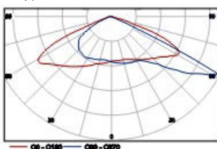
TypeIII Photometric curve
