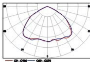
TypeV Photometric curve
