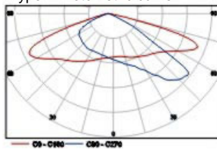
TypeII Photometric curve
