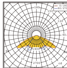
Lamp:65W LED
