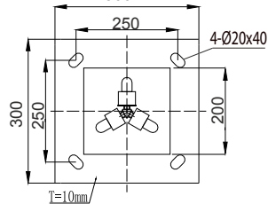
250*250mm column 350
