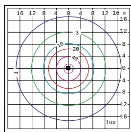
Moughing Height:4m
