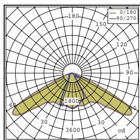
Lamp:80W LED
