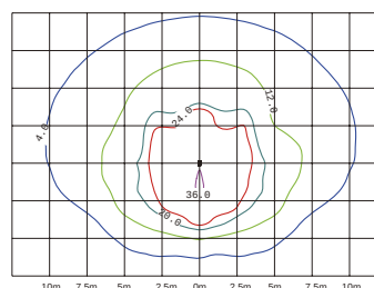
Lamp:50W LED Height 5m
