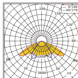
TypeIII Photometric curve
