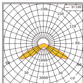
TypeV Photometric curve
