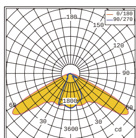
TypeI Photometric curve
