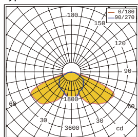
TypeII Photometric curve
